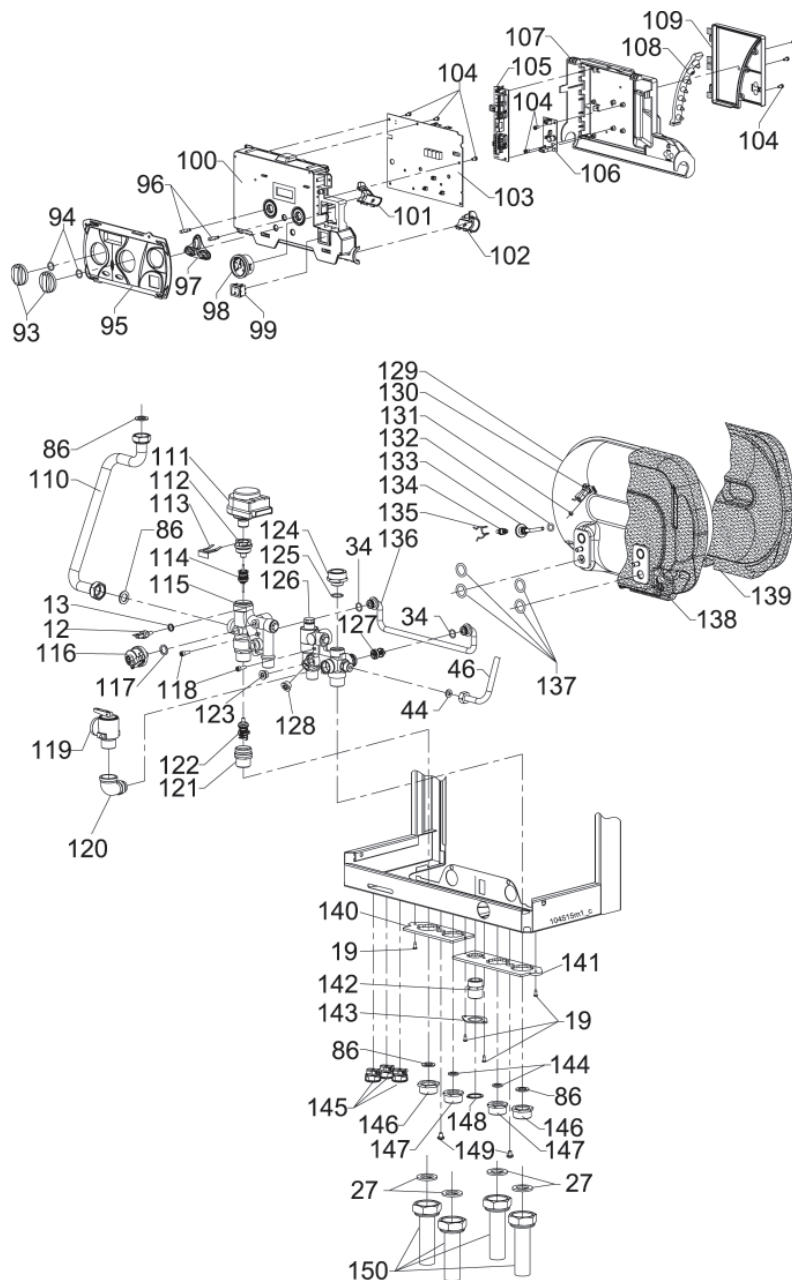
Bottom of the boiler for 160C and 160OC models
