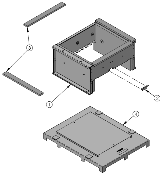
Base/Combustible Floor Pan
