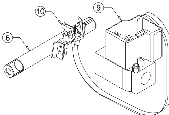
Gas Valve and Pilot Intermittent Ignition
