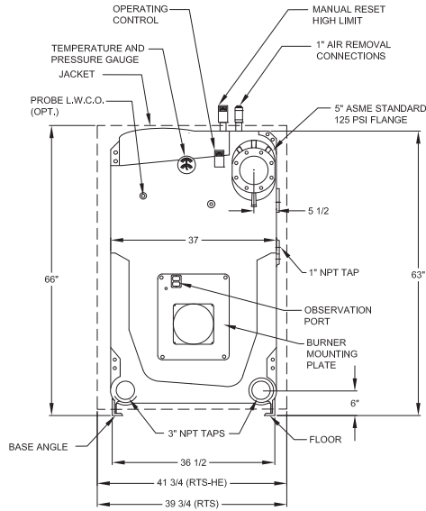
FRONT VIEW (Water Boiler)
