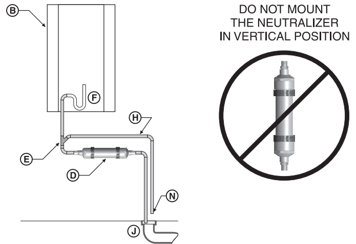
Figure 5 Y-fitting by-pass with wall-mounted boiler (see legend at left)
